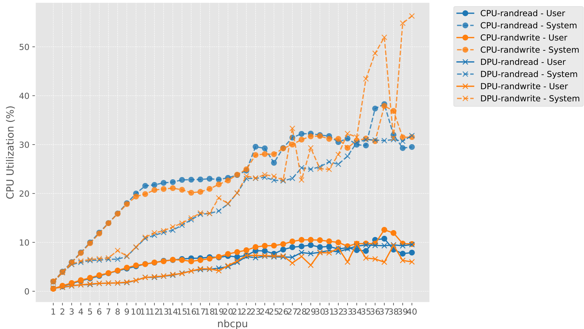
CPU Utilization vs nbcpu (CPU vs DPU)
